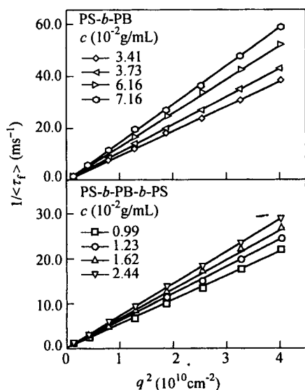
Fig. 4 Scattering vector ( q ) dependence of average characteristic decay time ( \langle\tau_f\rangle ) of fast relaxation for diblock and triblock chains in semidilute toluene solution
