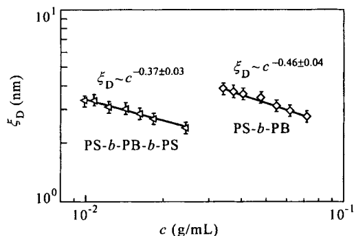
Fig. 6 Copolymer concentration dependence of dynamic correlation length ( \xi_D ) for diblock and triblock chains in semidilute toluene solution, where the definition of \xi_D can be found in the text
