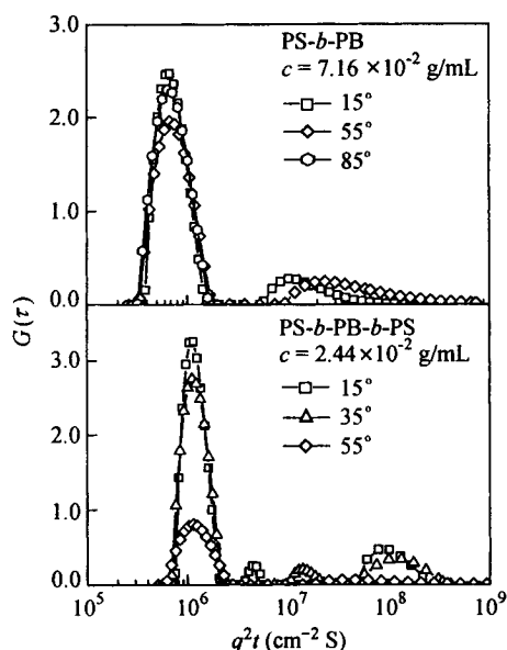
Fig. 3 Scattering angle dependence of characteristic decay time distribution G(\tau) of diblock and triblock chains in toluene for a given concentration well above the overlap concentration ( c^* \sim 1.5 \times 10^{-2} g/mL for \text{PS}_{210}\text{-}b\text{-PB}_{960} or \sim 1.2 \times 10^{-2} g/mL for \text{PS}_{200}\text{-}b\text{-PB}_{1815}\text{-}b\text{-PS}_{200} )
