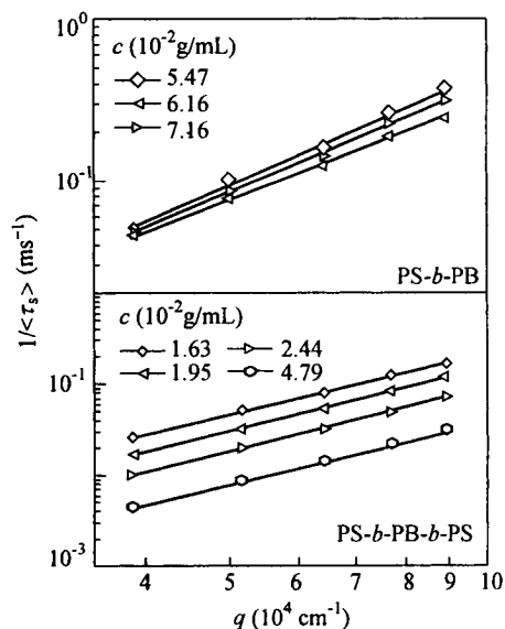
Fig. 5 Scattering vector ( q ) dependence of average characteristic decay time ( \langle\tau_s\rangle ) of slow relaxation for diblock and triblock chains in semidilute toluene solution
