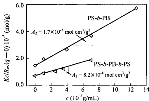
Fig. 7 Concentration dependence ( c ) of Rayleigh ratio ( R_w(q \rightarrow 0) ) for diblock and triblock chains in dilute toluene solution, where K is a constant defined in the text
