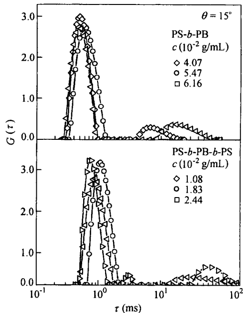
Fig. 2 Concentration dependence of characteristic decay time distribution G(\tau) of diblock and triblock copolymers in toluene
